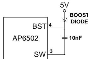
Figure 4—External Bootstrap Compensation Components
